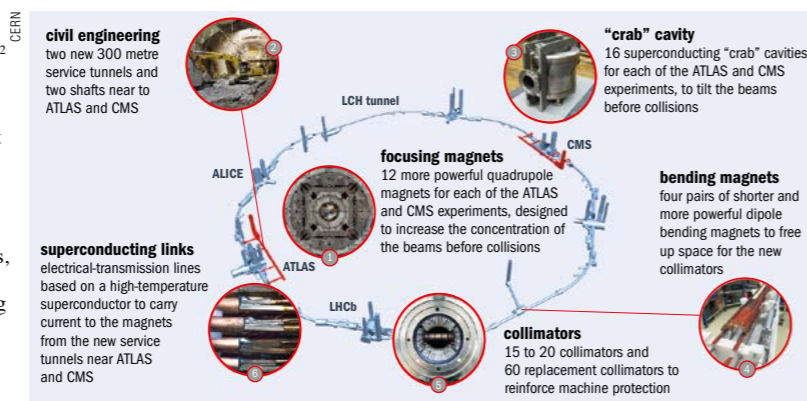
New technologies for the high-luminosity LHC.
