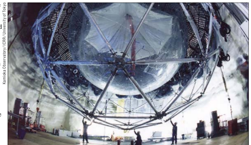
Top: The Super-Kamiokande Detector. Above: View of the SNO detector under construction.
