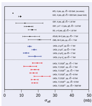
Summary of all available measurements of the \sigma_{eff} parameter.
