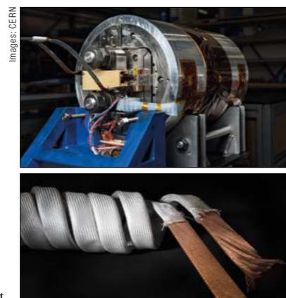
Top: The RMC_03 racetrack test magnet. Above: Samples of the two cables used to wind the RMC_03 coils.
