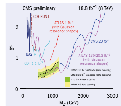
Upper limit of the coupling of a Z' B resonance as a function of its mass. The results are compared with results obtained by standard data-taking, as well as with similar searches at different colliders.
