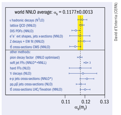
Summary of the strong coupling extractions discussed in the workshop.
