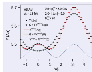
Template fit to the Y(\Delta\phi) in 13 TeV pp collisions for charged particle pairs with 0.5 < p_T^{a,b} < 5 GeV and 2 < |\Delta\eta| < 5 . This plot corresponds to the N_{ch}^{rec} \geq 90 interval. The open points indicate F Y^{periph}(\Delta\phi) + G (where G is the magnitude of the combinatoric component of the yield Y^{ridge} ), while the solid and dashed curves show the full template functions and Y^{ridge}(\Delta\phi) + F Y^{periph}(0) , respectively. The horizontal short-dashed line indicates G + F Y^{periph}(0) .
